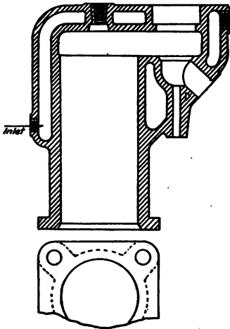
FIG. 5.—Water Cooled, Four Cycle Cylinder.
